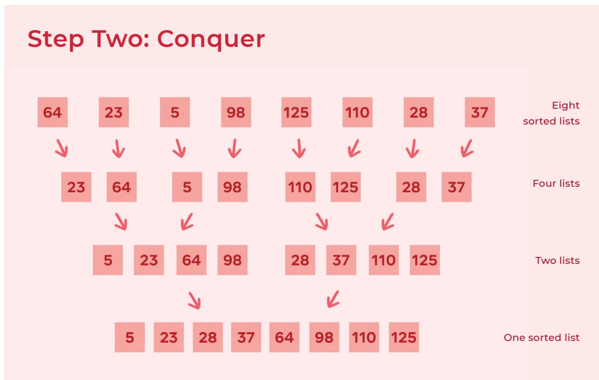
Merge Sort Diagram - Step Two: Conquer
