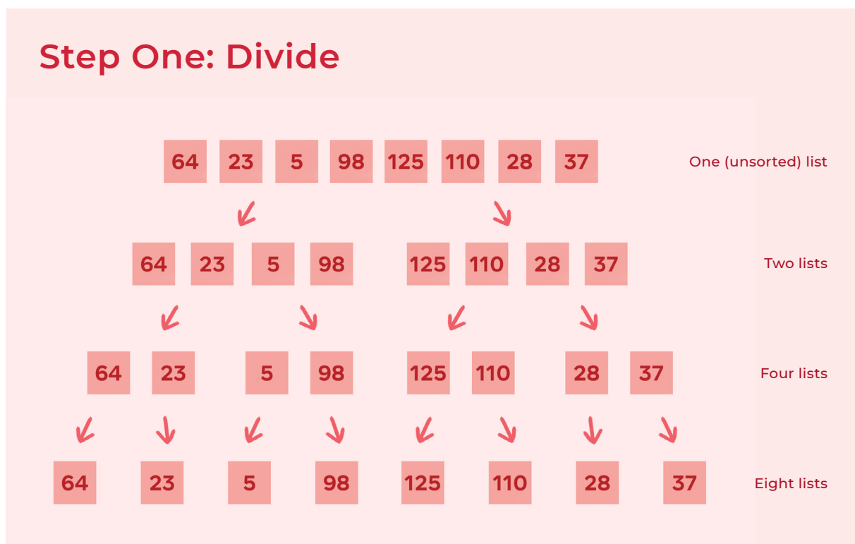
Merge Sort Diagram - Step One: Divide
